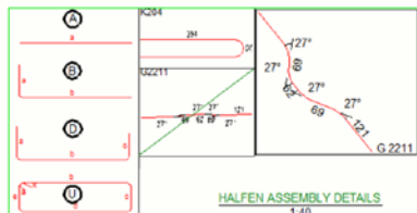
HALFEN ASSEMBLY DETAILS 1:40
