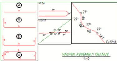
HALFEN ASSEMBLY DETAILS 1:40
