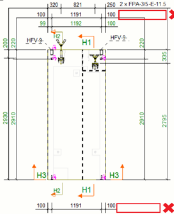
HALFEN ASSEMBLY DETAILS 1:40
